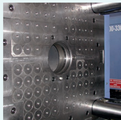
Pressmag SP on a 3000 kN (300 t) machine
